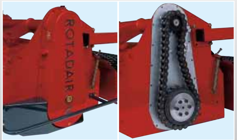
Double rotor drive with hydraulic torque limiting systems at both rotor ends guarantees protection, reliability and long service (RX 220/250/300).
